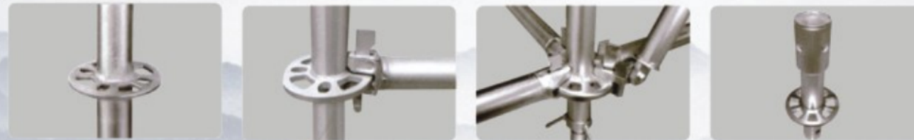
Diagonal Brace
